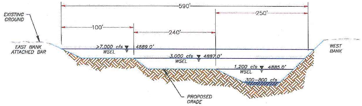
CONCEPTUAL CROSS-SECTION VIEW NOT TO SCALE
